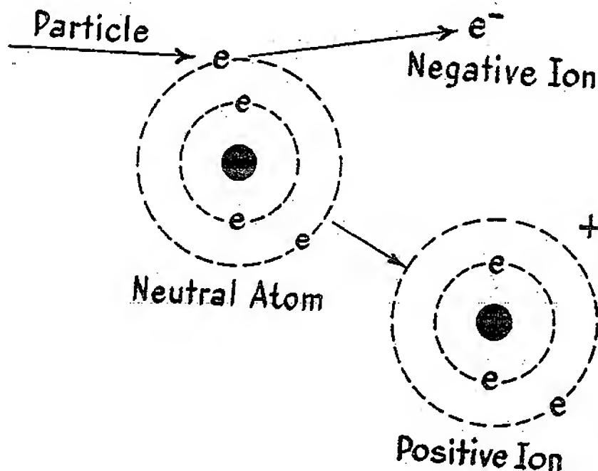
Figure 7—Ionization.
